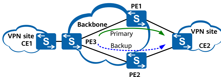
Figure 7-1 VPN FRR networking
