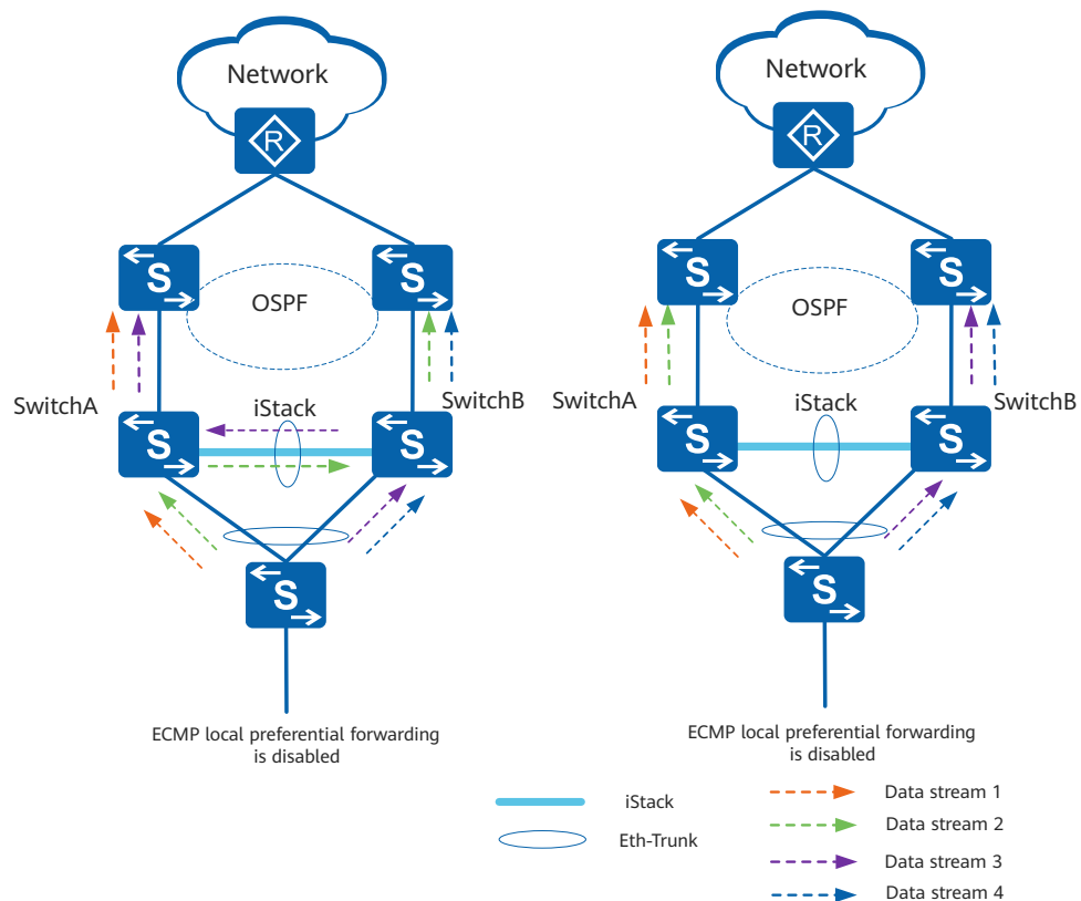
Figure 7-2 ECMP local preferential forwarding
