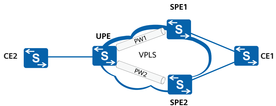
Figure 10-2 VPLS PW redundancy networking
