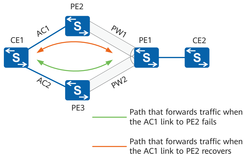
Figure 10-1 CE dual-homing to a VPLS network
