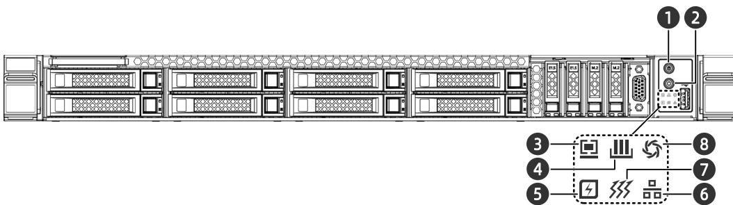
Figure 5-12 Front Panel LEDs and Buttons of 8 × 2.5-inch Drive + 2 × E1.S SSD + 2 × M.2 SSD Configuration
