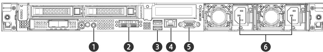
Figure 5-28 Rear Panel Ports 3
