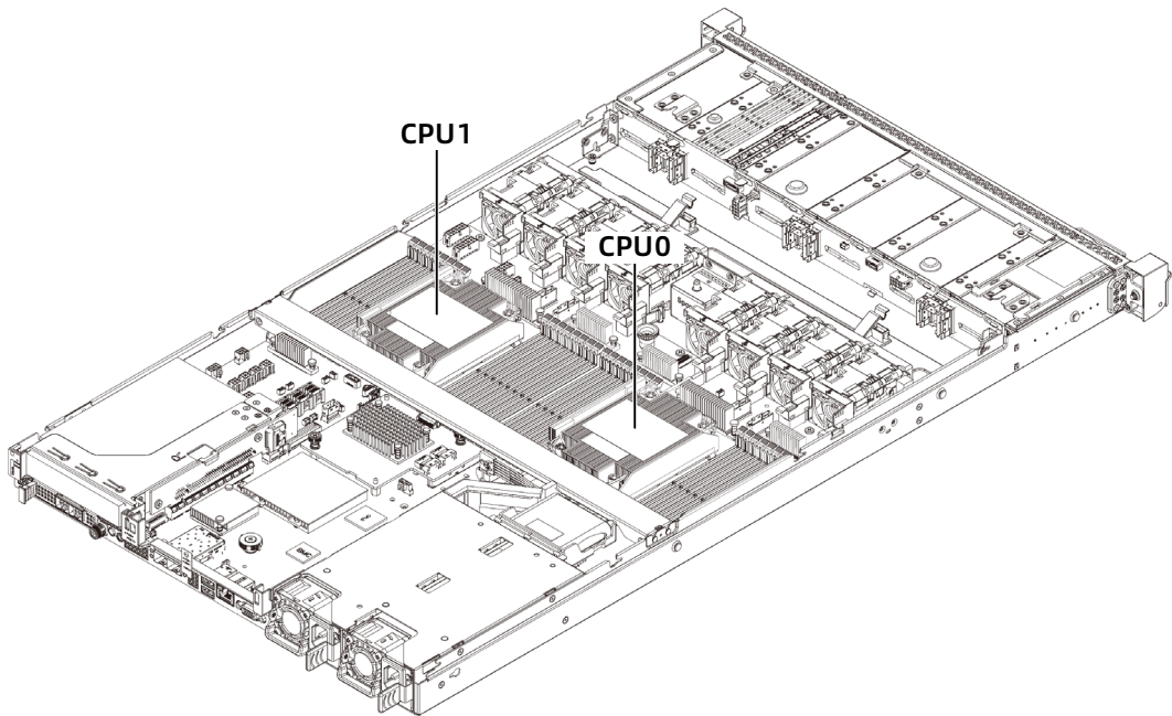
Figure 5-29 Processor Locations
