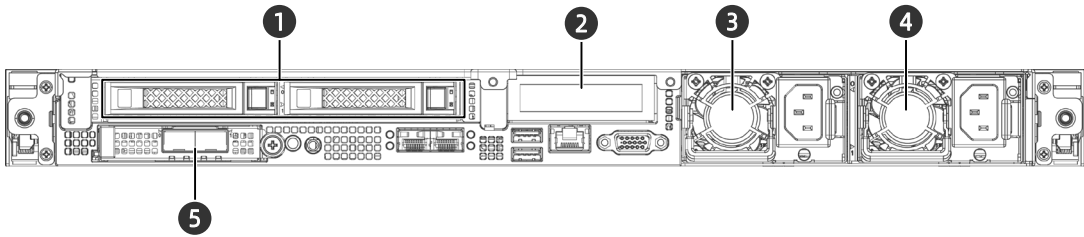
Figure 5-22 Rear View 3
