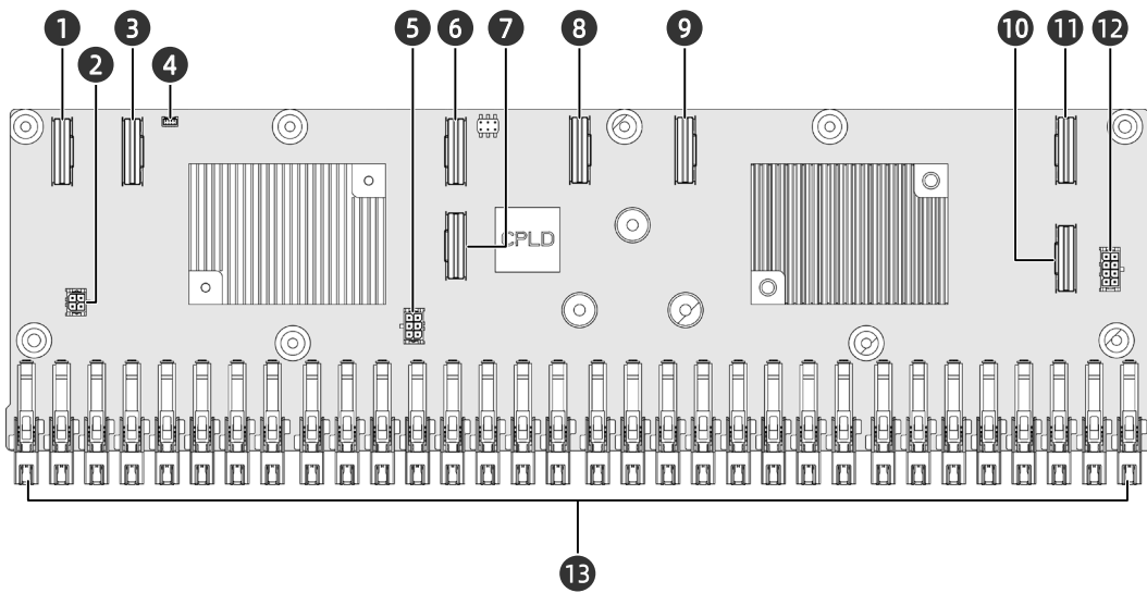
Figure 5-65 32 × E1.S SSD Drive Backplane
