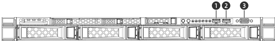
Figure 5-15 Front Panel Ports of 4 × 3.5-inch Drive + 2 × E1.S SSD + 2 × M.2 SSD Configuration
