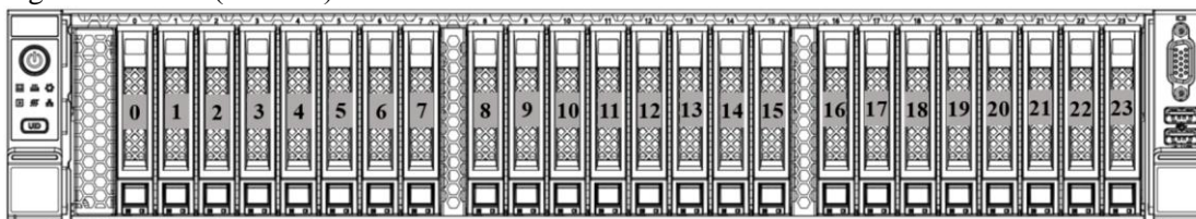
Figure 7-3 Front 25 × 2.5"
