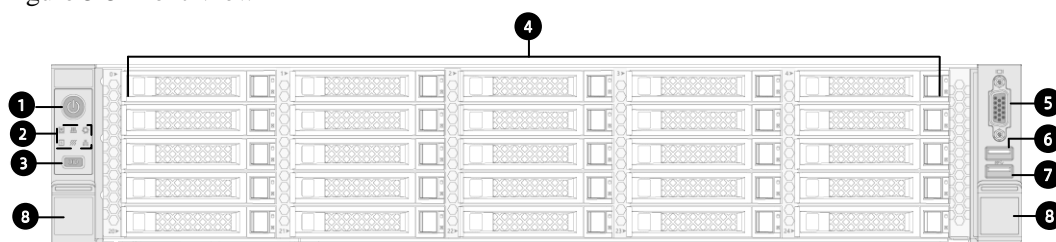
Figure 5-5 Front View
