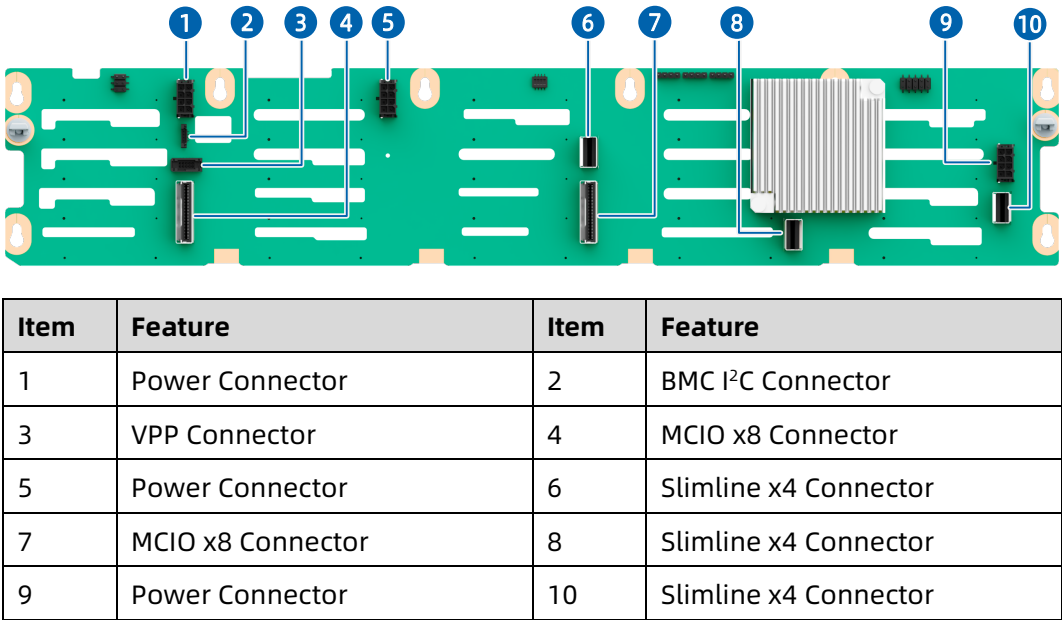
Figure 5-43 25 × 2.5-Inch Drive Backplane
