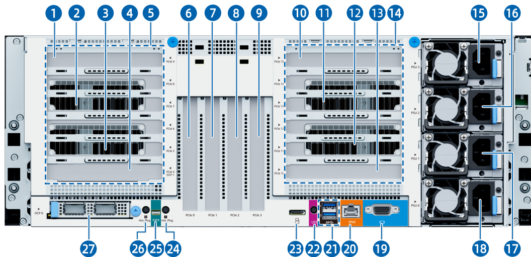
Figure 5-8 Rear View
