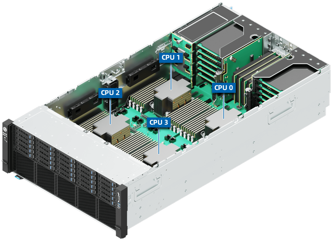
Figure 5-11 Processor Locations
