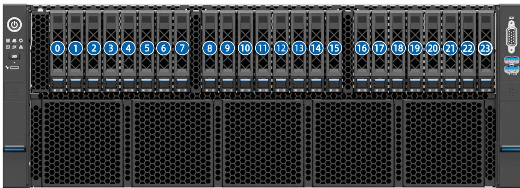
Figure 5-17 Drive Numbering
