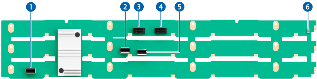
Figure 5-37 12 × 3.5-Inch Drive Backplane
