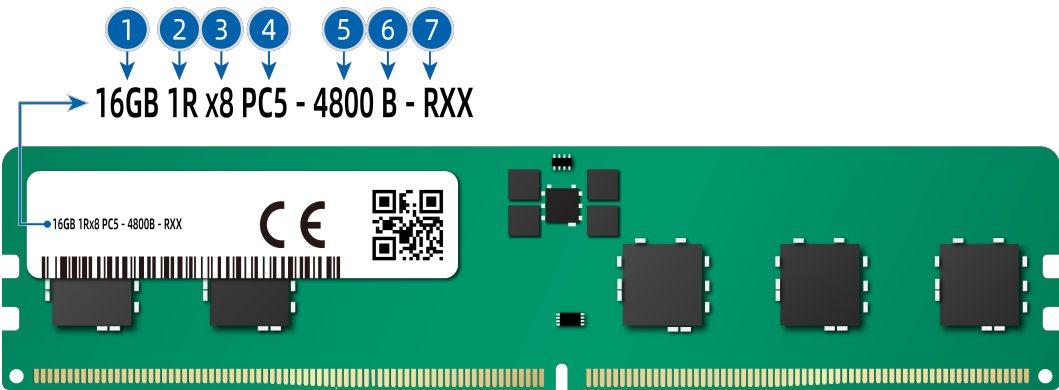
Figure 5-12 DIMM Identification
