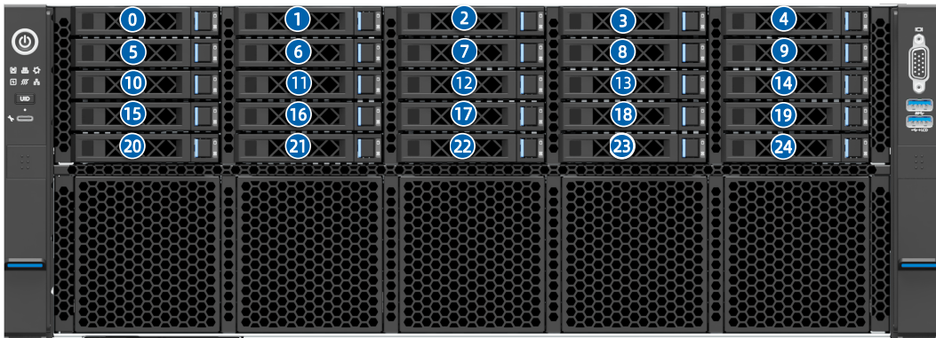
Figure 5-18 Drive Numbering
