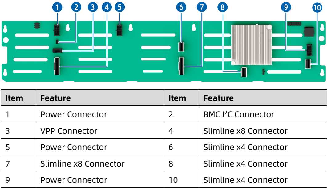
Figure 5-42 25 × 2.5-Inch Drive Backplane
