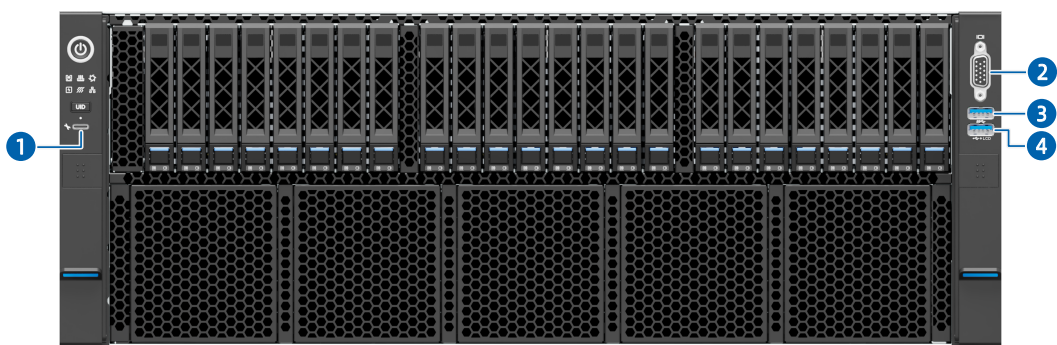
Figure 5-5 Front Panel Port Locations
