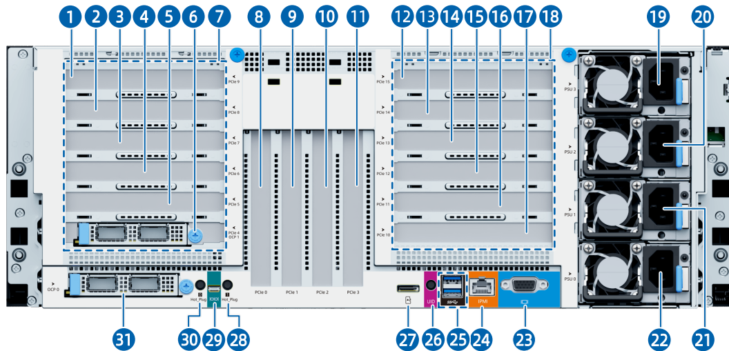
Figure 5-7 Rear View
