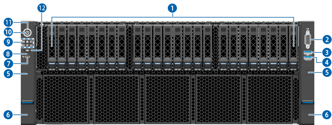
Figure 5-1 Front View
