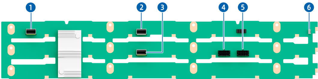
Figure 5-38 12 × 3.5-Inch Drive Backplane
