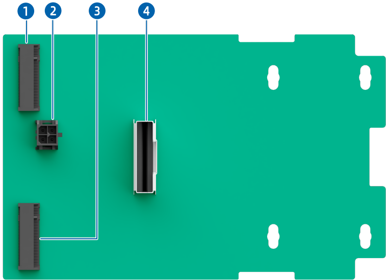
Figure 5-45 M.2 Adapter
