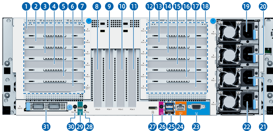
Figure 5-6 Rear View
