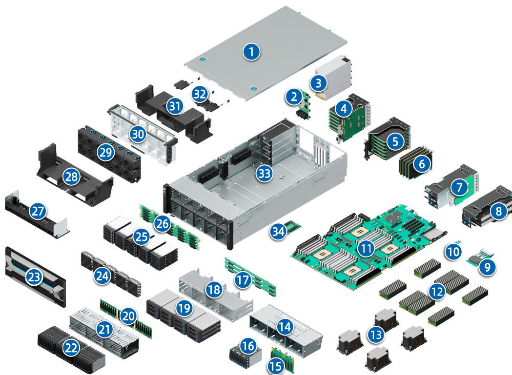
Figure 3-1 Exploded View
