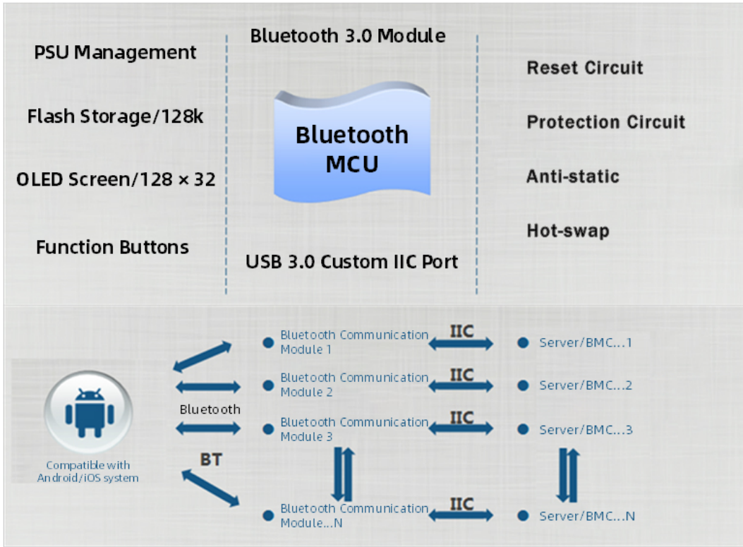
Figure 5-31 How LCD Subsystem Works
