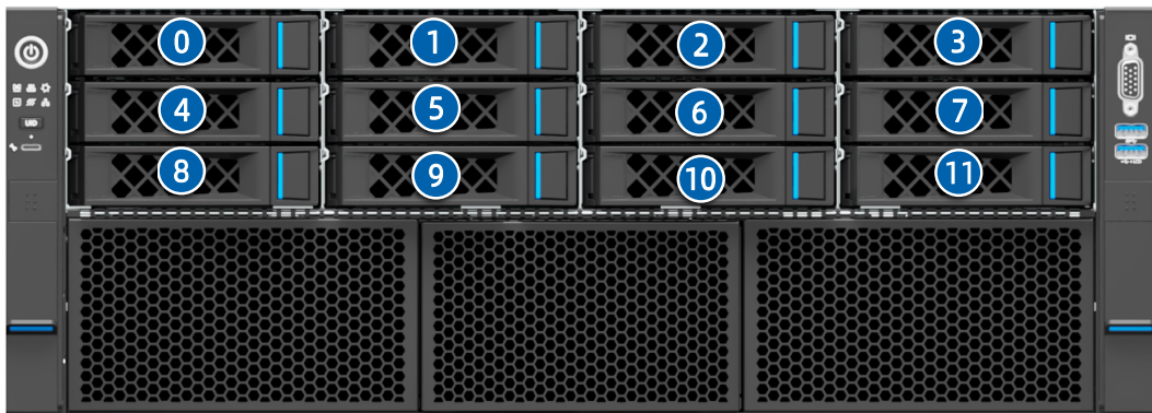
Figure 5-19 Drive Numbering
