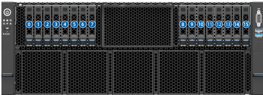
Figure 5-16 Drive Numbering
